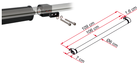
Kit Roof Rail Ducato Extra (x2)
