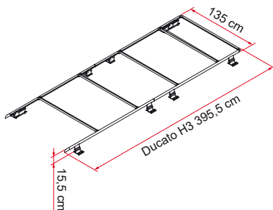
Kit Roof Rail Ducato Extra (x2)
